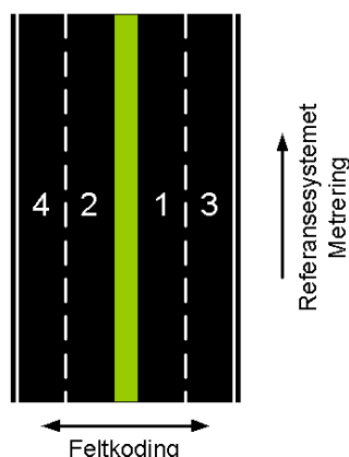
Figur 21 Feltkoding
